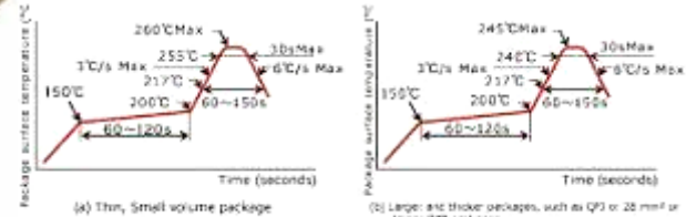
Figure 4.14 Reflow Heat Resistance Temperature Profiles for IPC/JEDEC Standards
