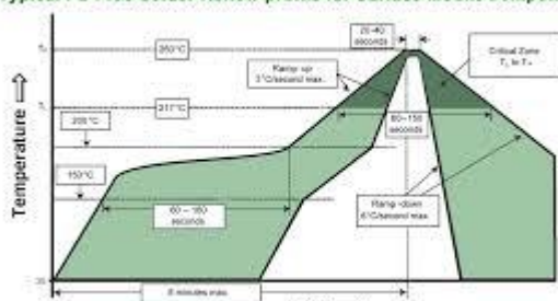
Profile Classification per IPC/JEDEC J-STD-020C Pb-Free Small Body Assembly Typical Pb-Free Solder Reflow profile for Surface Mount Components
